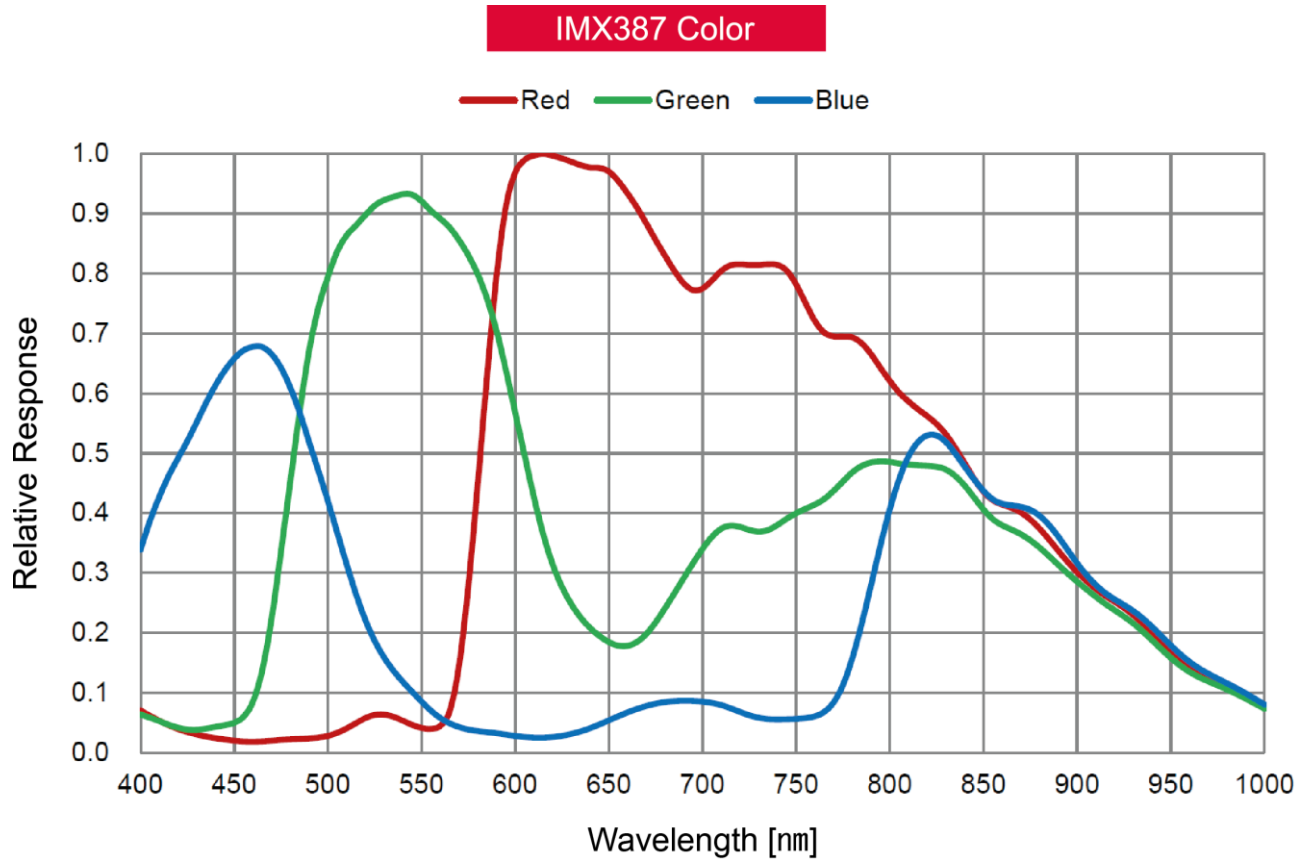
Figure 5.4 VC-17MC-C48 H Spectral Response
