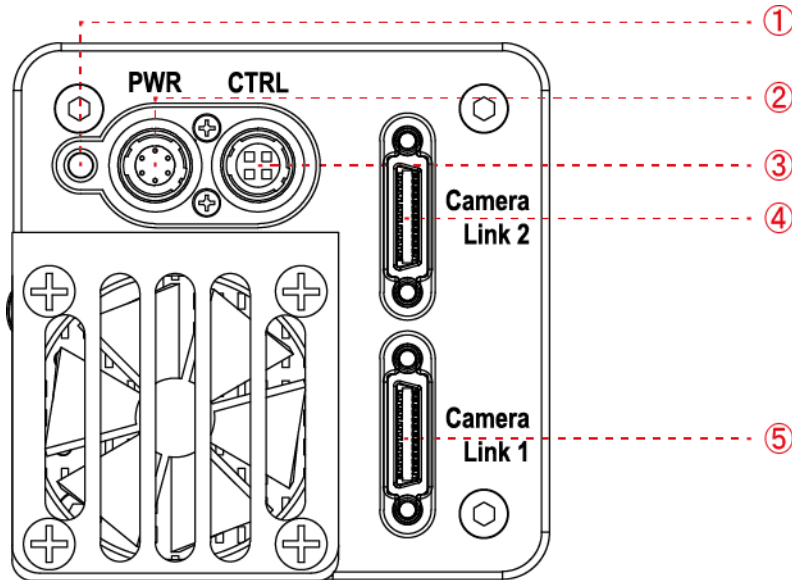
Figure 7.1 VC-17MC-48 H / VC-31MC-26 H 뒷면 패널
