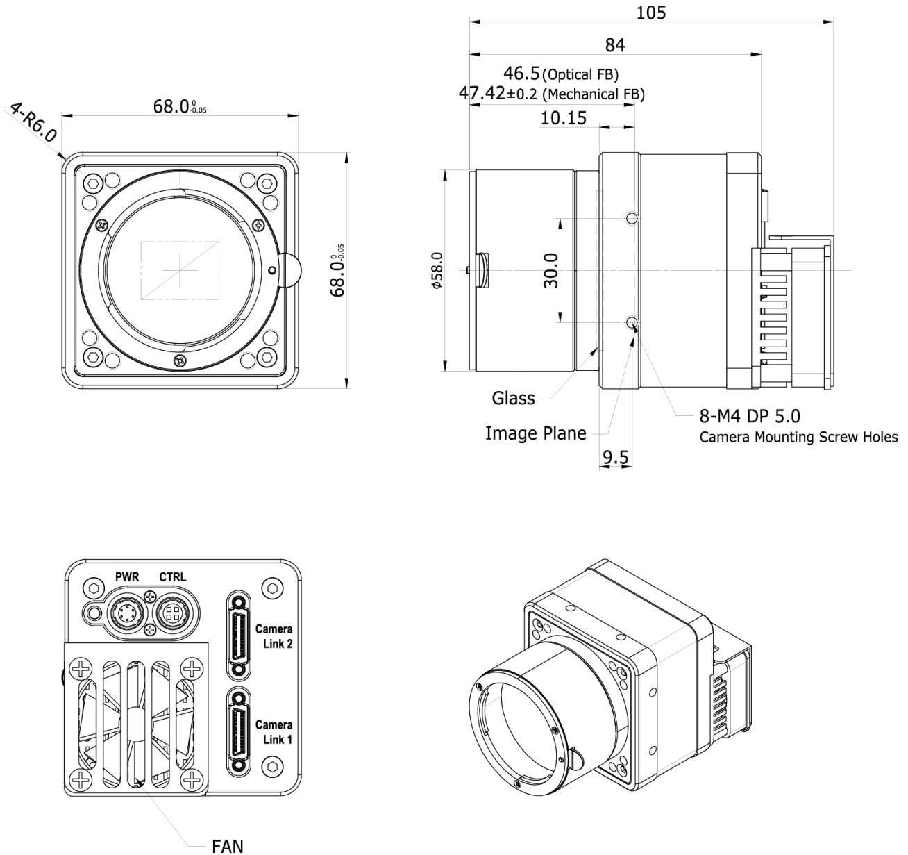
Figure 5.6 VC-17MC-48 H 및 VC-31MC-26 H F-mount Mechanical Dimension
