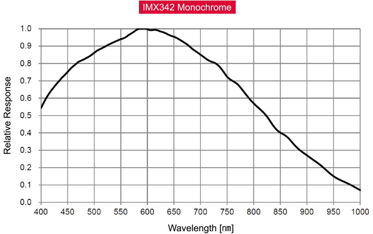
Figure 5.3 VC-31MC-M26 H Spectral Response
