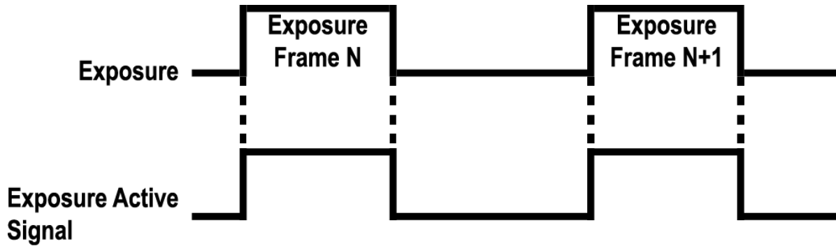
Figure 9.18 Exposure Active Signal
