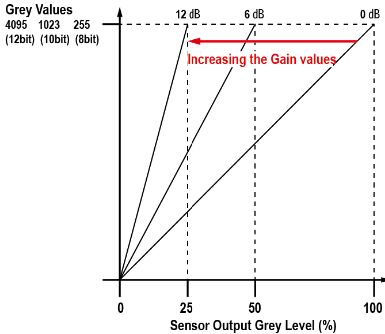
Figure 9.7 Gain 설정
