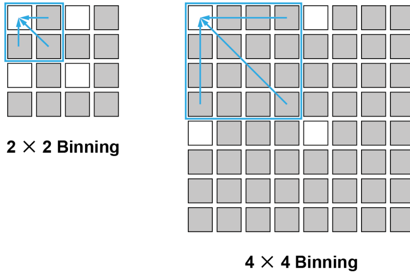
Figure 9.3 2 × 2 및 4 × 4 Binning
