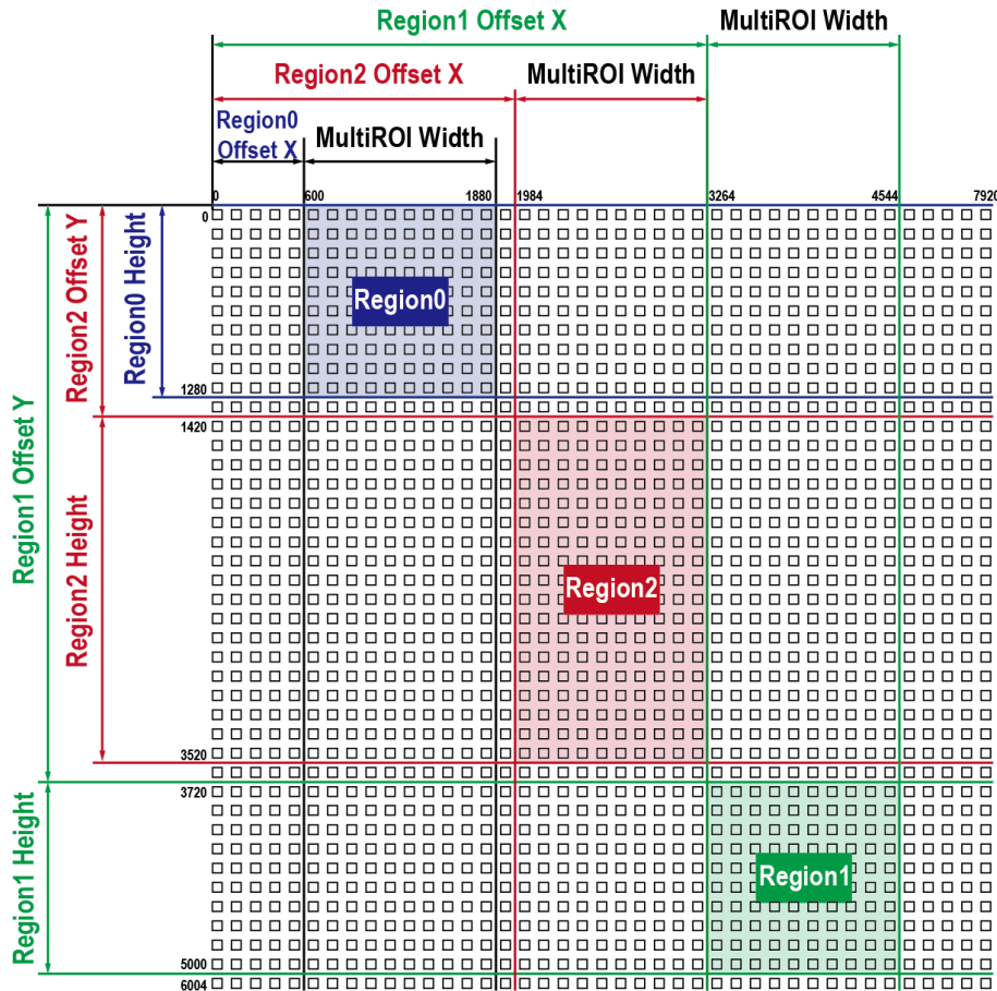
Figure 9.2 Multi-ROI
