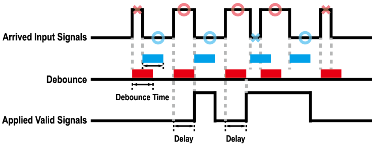
Figure 9.19 Debounce
