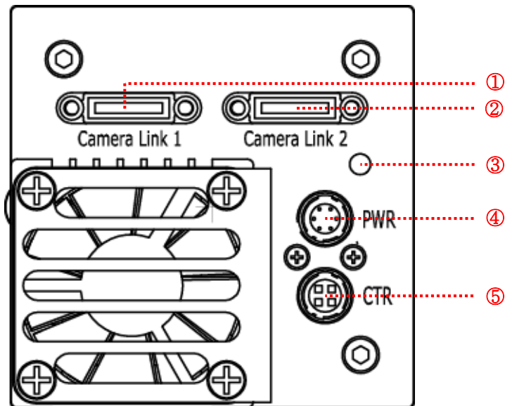
Figure 7.1 VC-71MC Camera 뒷면 패널
