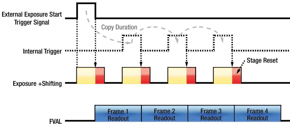
Figure 9.14 Sequence 4 shot 모드에서 Multi Shot Enable일 때 Timing Diagram
