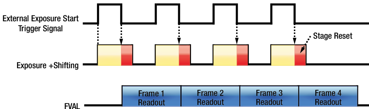
Figure 9.15 Sequence 4 shot 모드에서 Multi Shot Disable일 때 Timing Diagram
