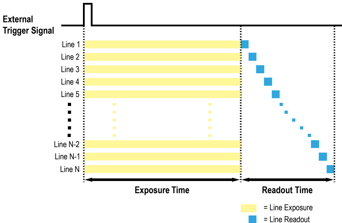
Figure 8.2 Global Shutter
