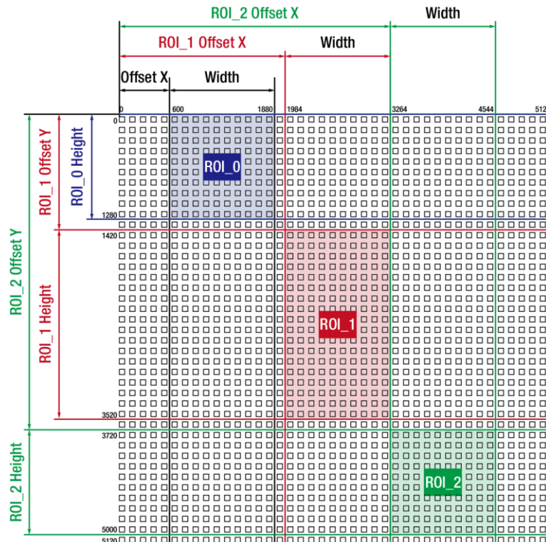
Figure 8.2 Multi-ROI
