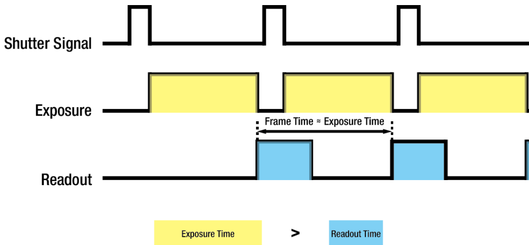
Figure 8.7 Exposure Time이 Readout Time보다 길 때
