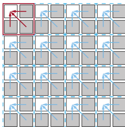
Figure 8.4 2 \times 2 Binning
