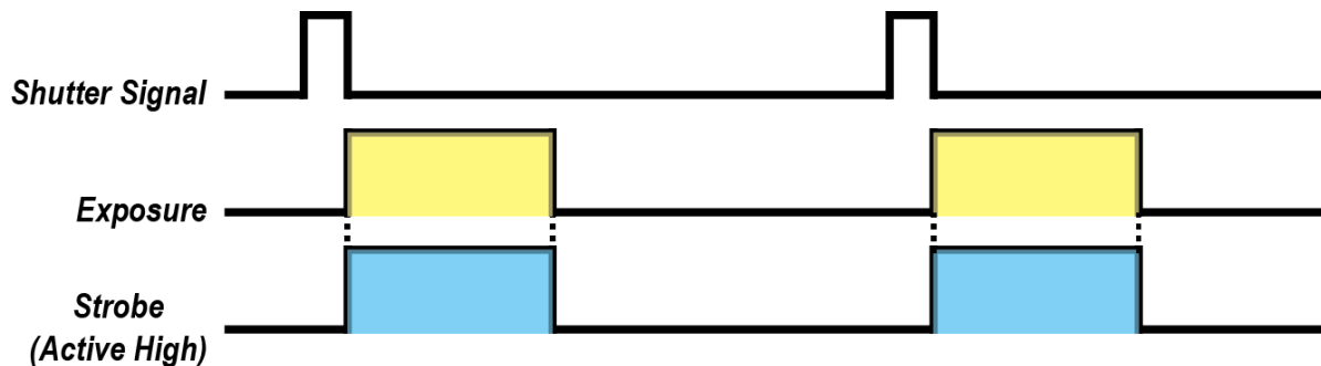
Figure 8.23 Strobe Output
