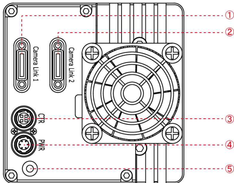
Figure 7.1 VP-25MC Camera 뒷면 패널
