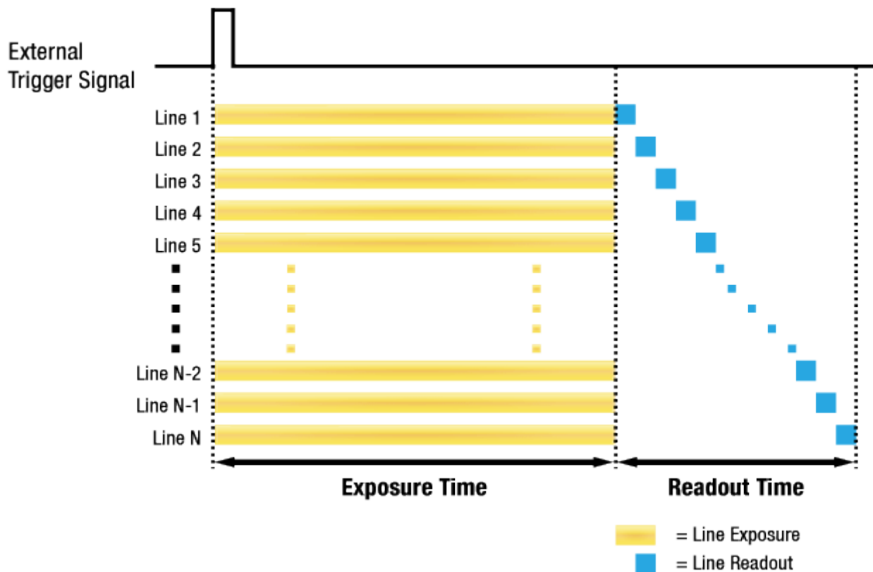
Figure 8.11 Global Shutter
