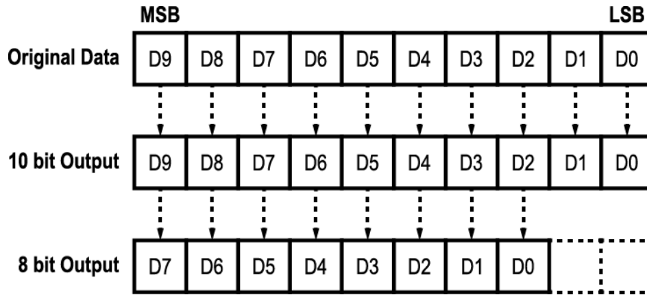
Figure 9.5 VC-65MX2-711 Pixel Format
