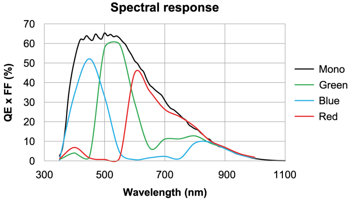
Figure 5.2 VC-65MX2-M/C711 Spectral Response
