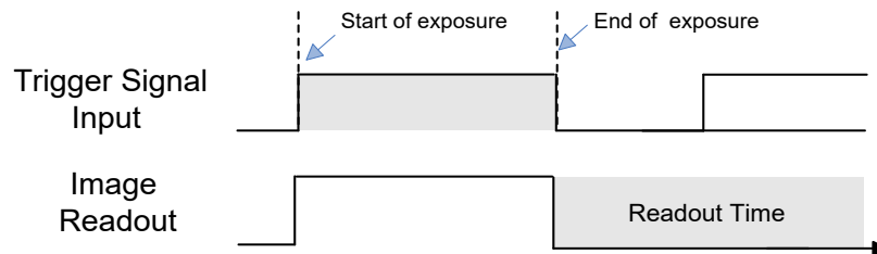
Figure 9-5 Exposure Timing Diagram
