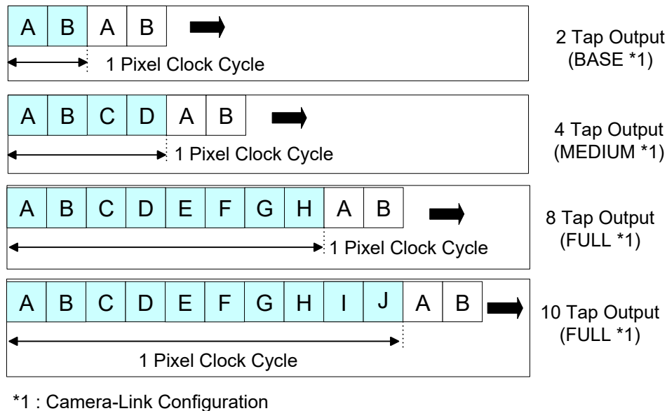
Figure 9-11 Camera Link Output Mode
