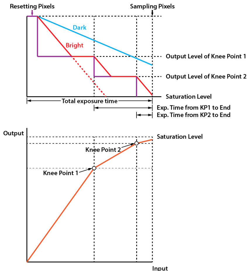
Figure 9-18 High Dynamic Range Concept Drawing
