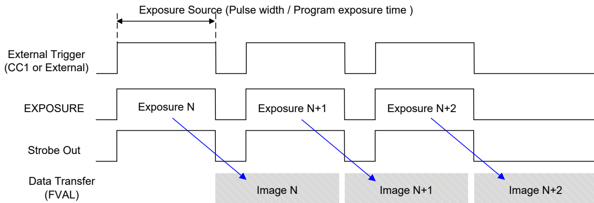
Figure 9-10 Camera Operation when Overlap Trigger is entered
