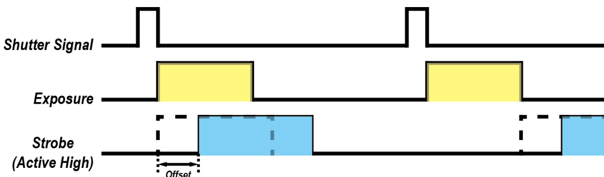
Figure 9-25 Strobe Offset
