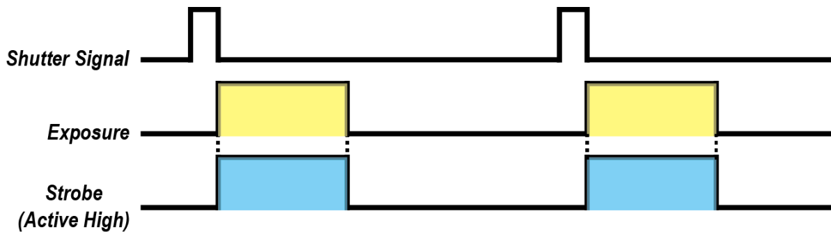
Figure 9-24 Strobe Output
