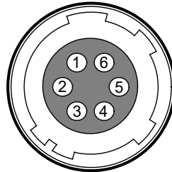
Figure 8-3 Pin Arrangement of Power Input Connector
