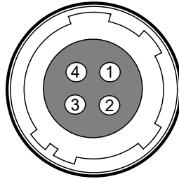
Figure 8-4 Pin Arrangement of Control Connector
