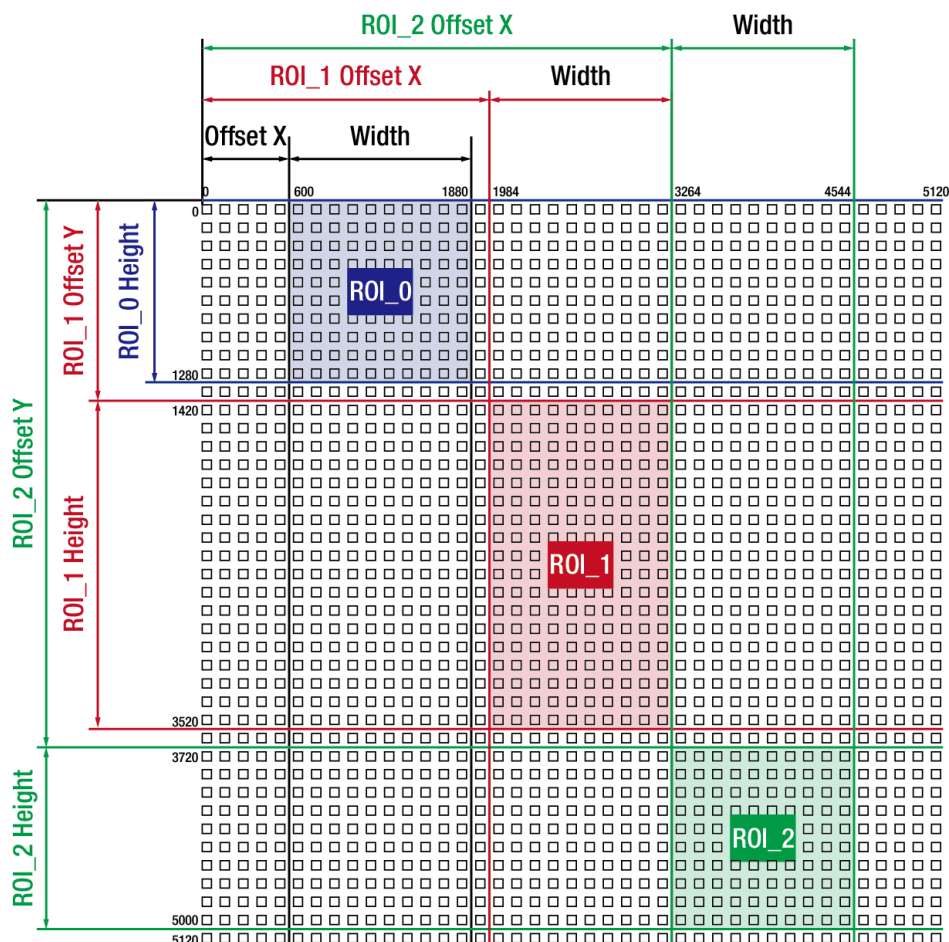
Figure 9-3 Multi-ROI (VC-25MC)
