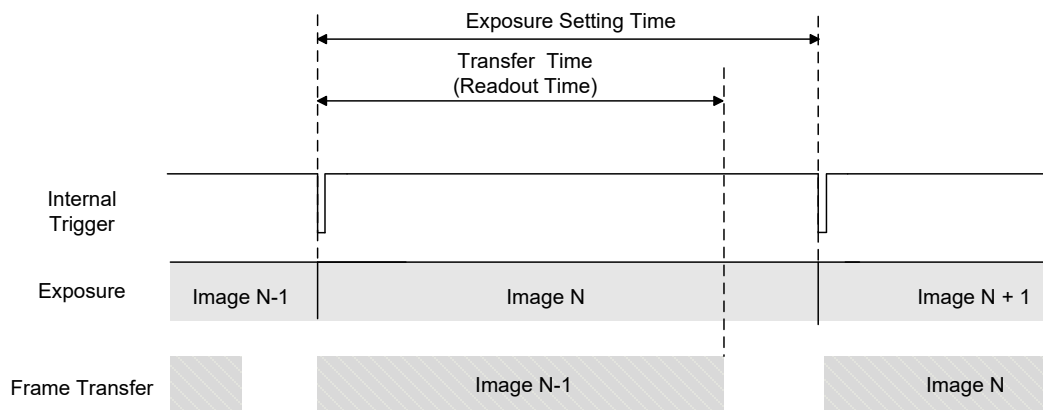
Figure 9-8 Exposure Time is longer than Readout Time
