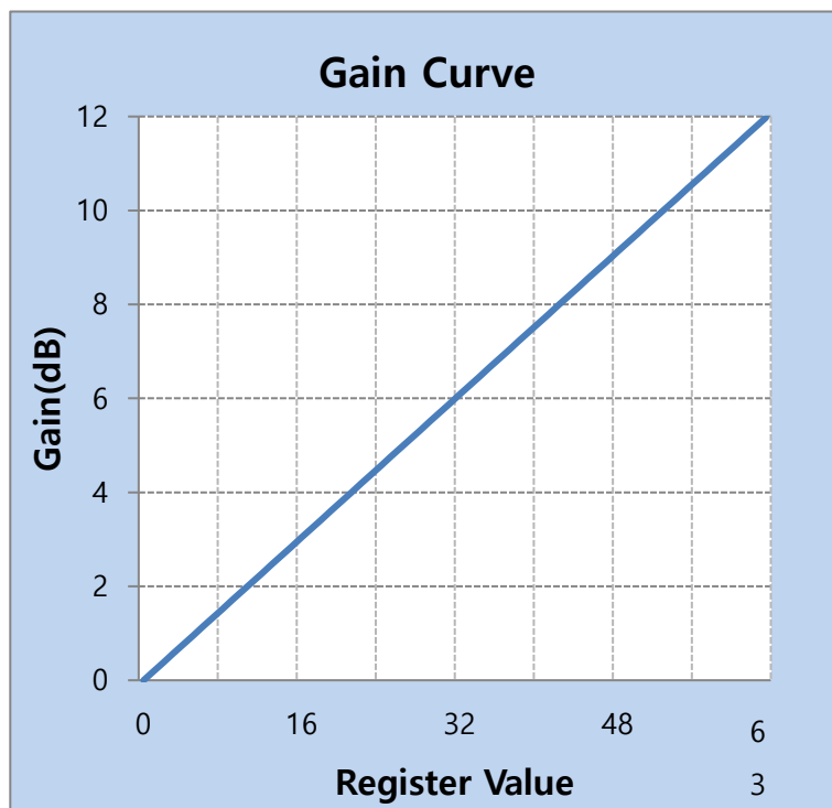
Figure 9-12 Register Setting vs Gain
