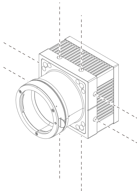
Figure 6-13 Locations available to Tighten the Setscrews when Mounting the Product
