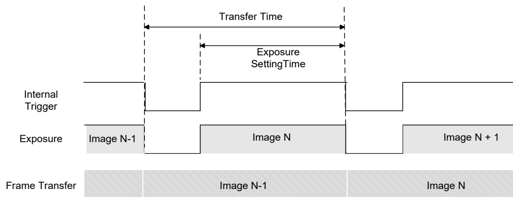
Figure 9-7 Exposure Time is shorter than Readout Time
