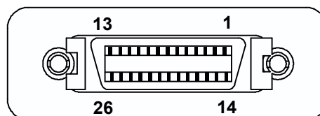
Figure 8-2 Camera Link Connector
