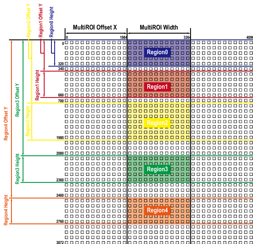
Figure 9.4 Multi-ROI(VC-12MX-M/C 180)
