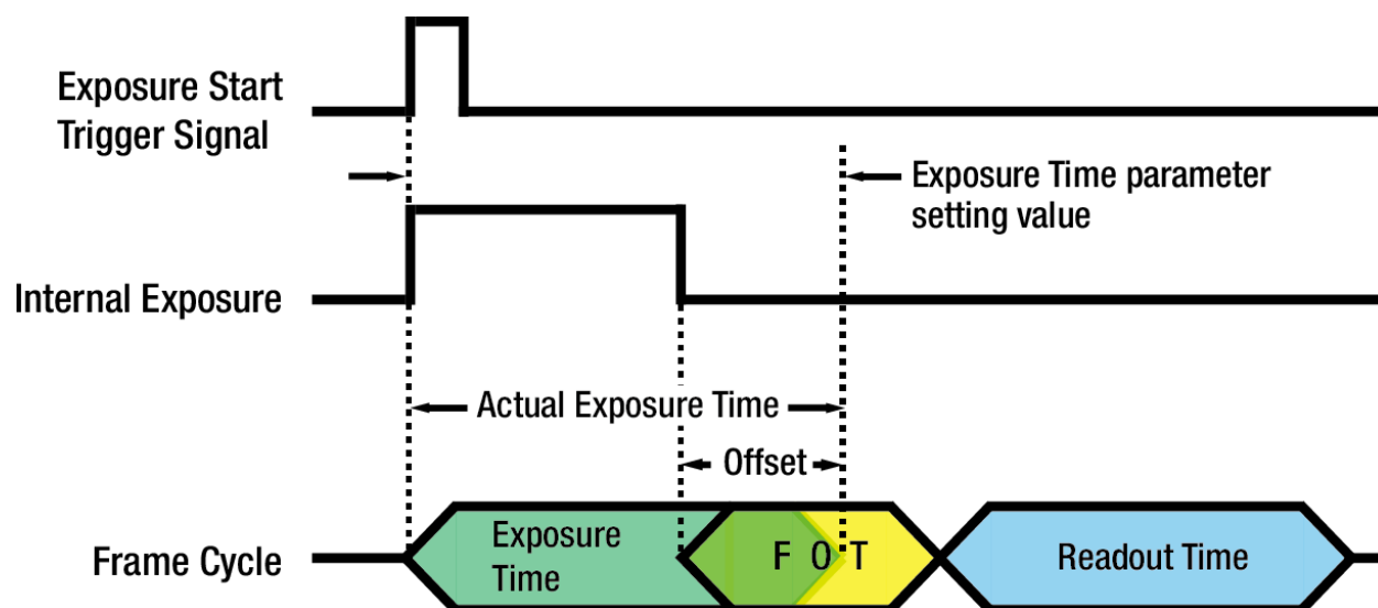
Figure 8.6 Real Exposure with Timed Exposure Mode
