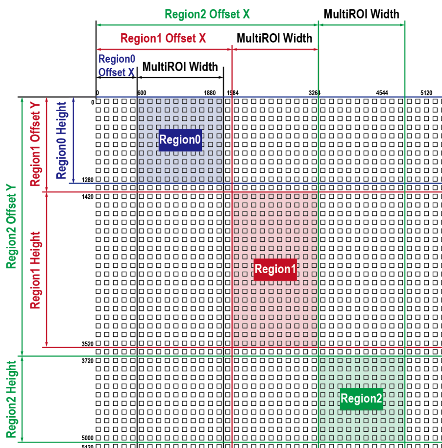
Figure 9.2 Multi-ROI(VC-25MX-81 D)
