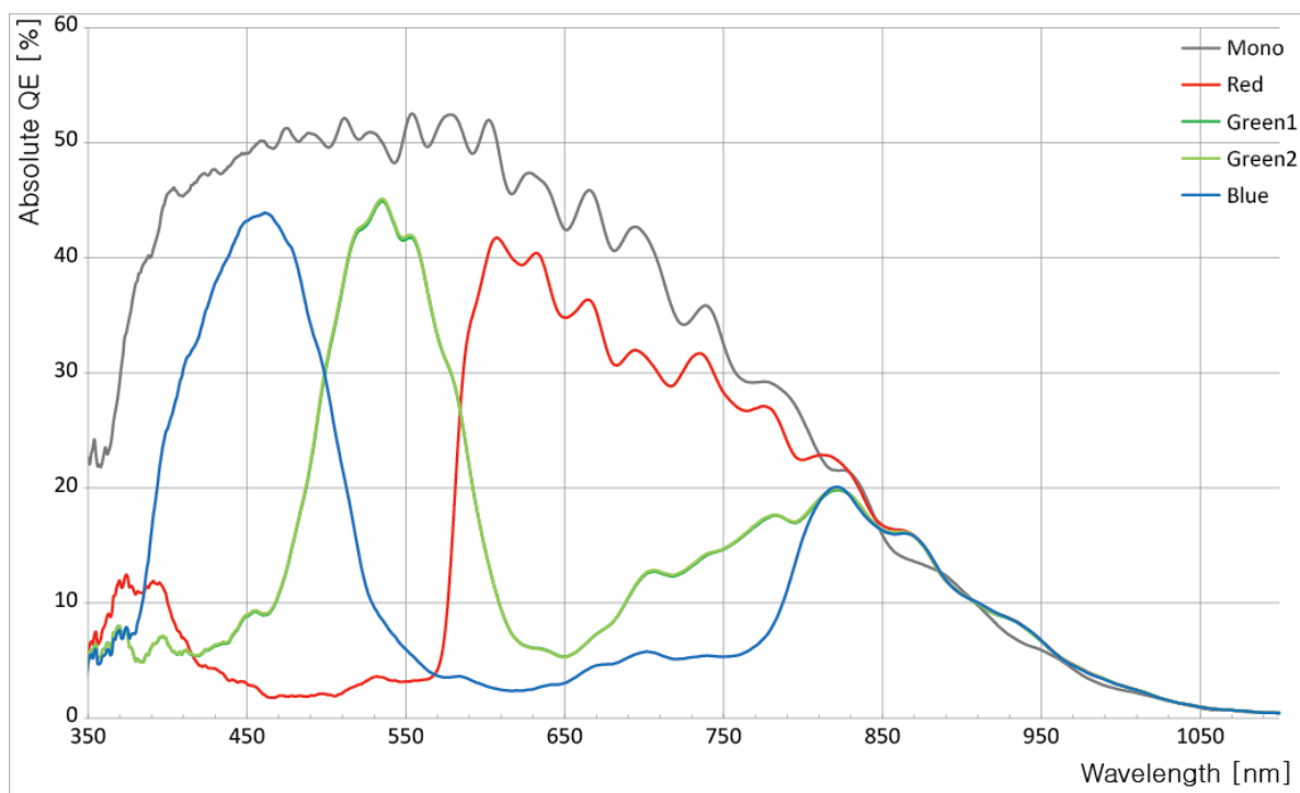
Figure 5.2 Mono and Color Spectral Response for VC-12MX-180
