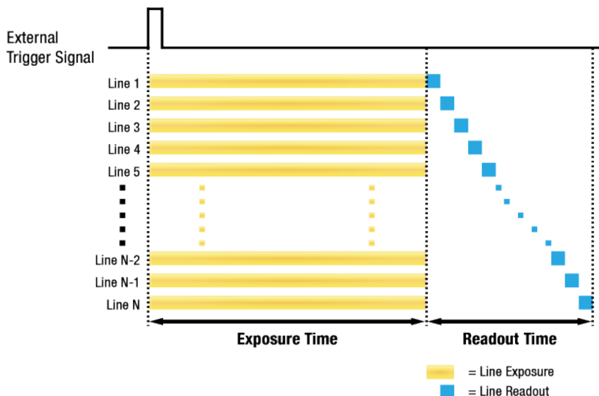
Figure 8.8 Global Shutter
