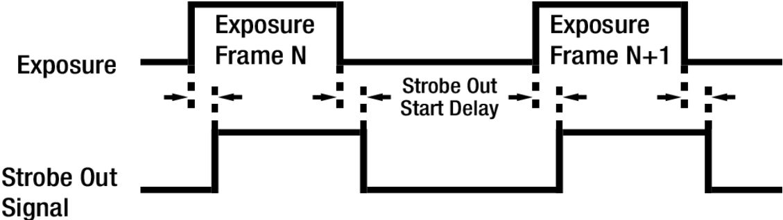
Figure 9.22 Strobe Out Signal
