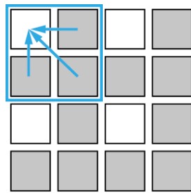
2 × 2 Binning
